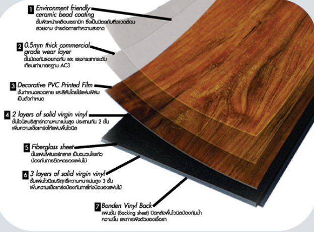
The picture below depicted the construction layers for allure locking
