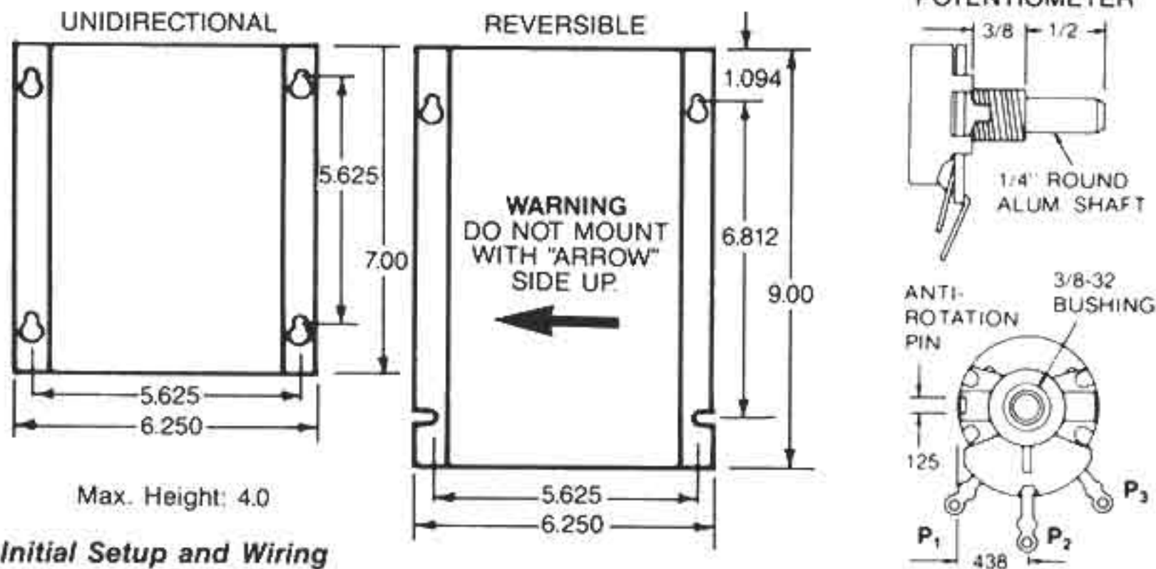
FIG. 2 MECHANICAL SPECIFICATIONS (inches)
