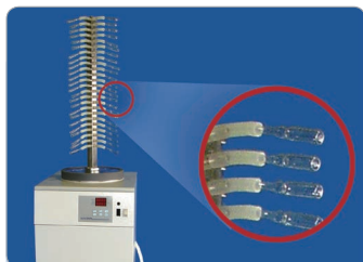
Ampoule manifold (Ampoule and rubber tube)
