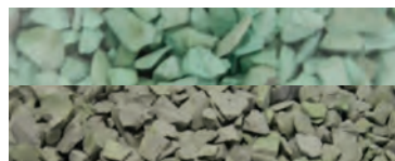
Oxygen Adsorbent: Top: Full Capacity; Bottom: Depleted.
